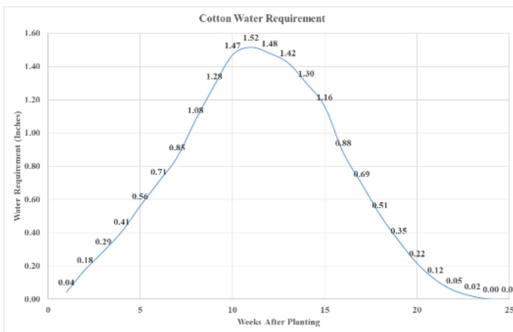
Figure 1. Weekly UGA Checkbook Cotton Irrigation for Full Season
