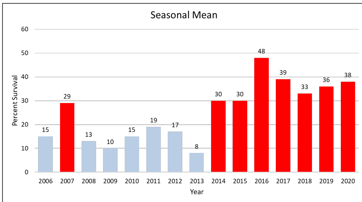
Figure 3. Seasonal mean survival of CEW in Adult Vial Tests (cypermethrin 5 µg/vial).
