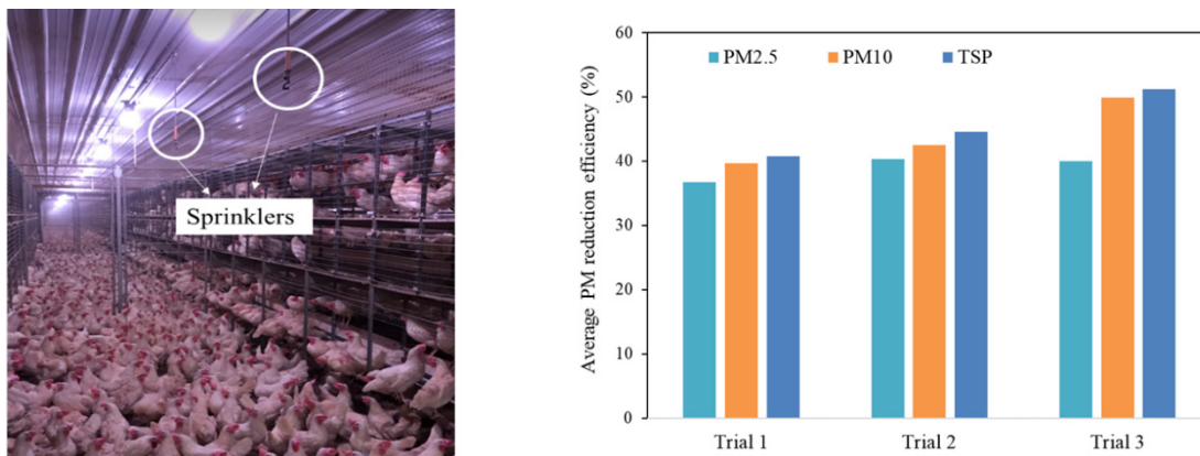
Figure 2. The sprinkler system (a) and dust reduction efficiency (b) (PM 2.5 and PM 10 refer to particulate matter smaller than 2.5 and 10 micrometers in diameter, respectively; TSP: total suspended particles) (Chai et al. , 2019).
